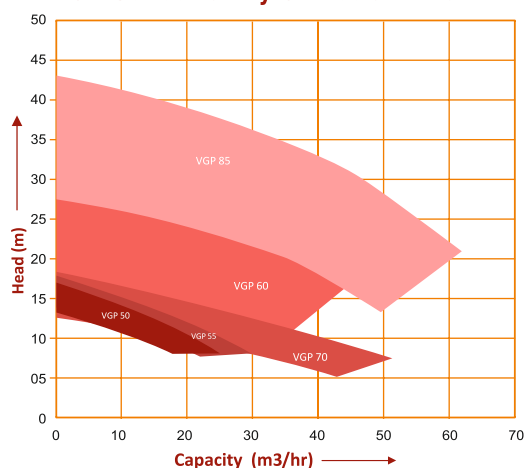
VGP Series Family Curves at 1440 RPM
