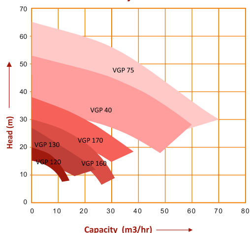
VGP Series Family Curves at 2880 RPM
